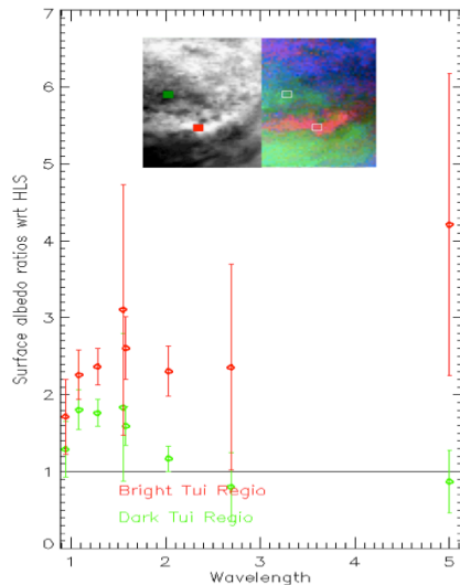
Figure 1: PCA on VIMS data (picture within plot - the red spot marks the bright area, the green the dark area) and retrieval of surface albedo ratios with RT between the bright and the dark Tui Regio RoIs with respect to the Huygens landing site albedo.
