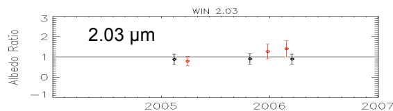
Figure 2. Time variation of Sotra Patera of the average surface albedo obtained within the 2.03 μm methane window. The red marks correspond to Sotra Patera data and the black ones to the test case dunes field centered at 172°W-7.5°S.
